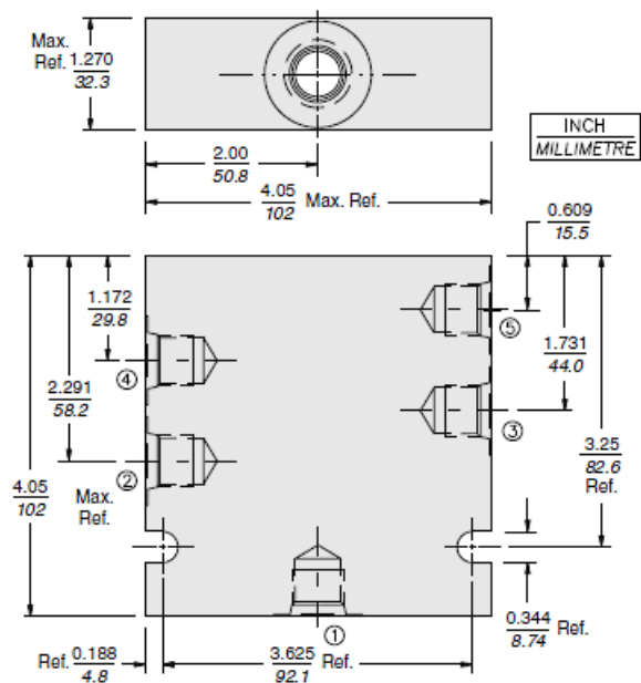
SAE 6 Ported Housing Shown
