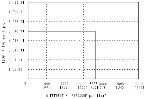
FLOW RATING vs DIFFERENTIAL PRESSURE
