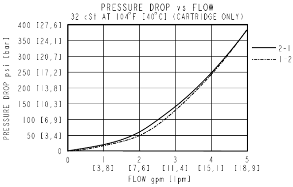
FLOW RATING vs DIFFERENTIAL PRESSURE
