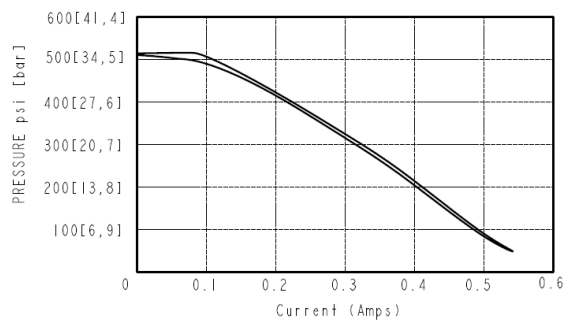
RELIEVING PRESSURE VS CURRENT CHARACTERISTIC (20V)
