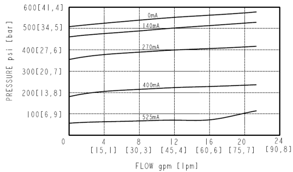
RELIEVING PRESSURE VS FLOW CHARACTERISTIC AT VARIOUS CONTROL CURRENTS (20V)
